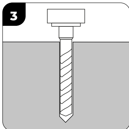
3 - Drill the hole with the 9/16" drill bit and 50 mm deep;
